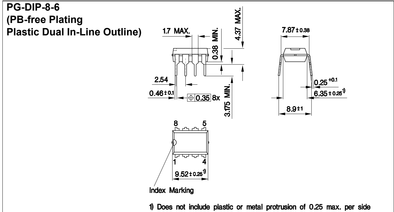
Figure 23 PG-DIP-8-6 (PB-free Plating Plastic Dual In-Line Outline)
